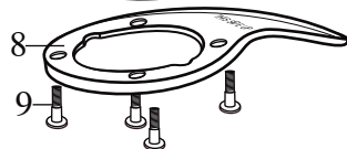
503341 S Blade Cutter Assembly (changed after 2/8/2010)
