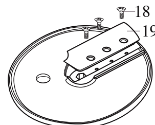
037339 (on units after 10/14/2019) 024171 1/2" Slicer (CAF18)
